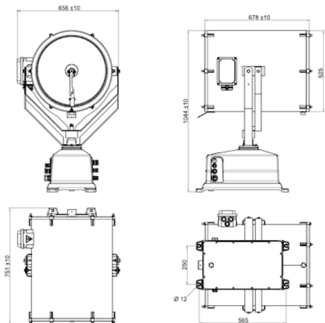
Images Measurement Drawing for SL40 R3 Xenon Searchlight for 2000Watt
