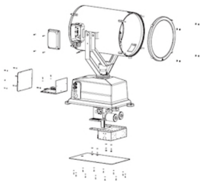
Explosion Drawing for SL40 R5 Xenon Searchlight
